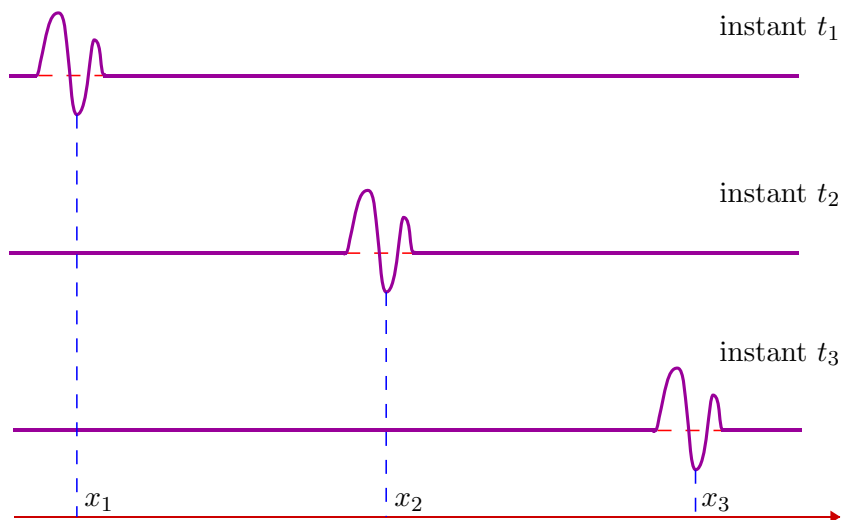
FIG. 1.3 – Onde progressive.
